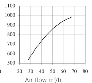
Power vs air flow @ RT (25°C)
