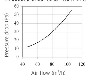
Pressure drop vs air flow @ RT (25°C)
