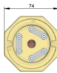
Delta connection D 3x400V
