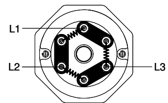
Delta connection D 3x400V
